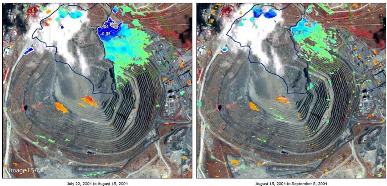
Figure 5: 2 months of pit movement - monitoring of ground subsidence occurring around Rio Tinto's Palabora mine in South Africa using Interferometric Synthetic Aperture Radar.
