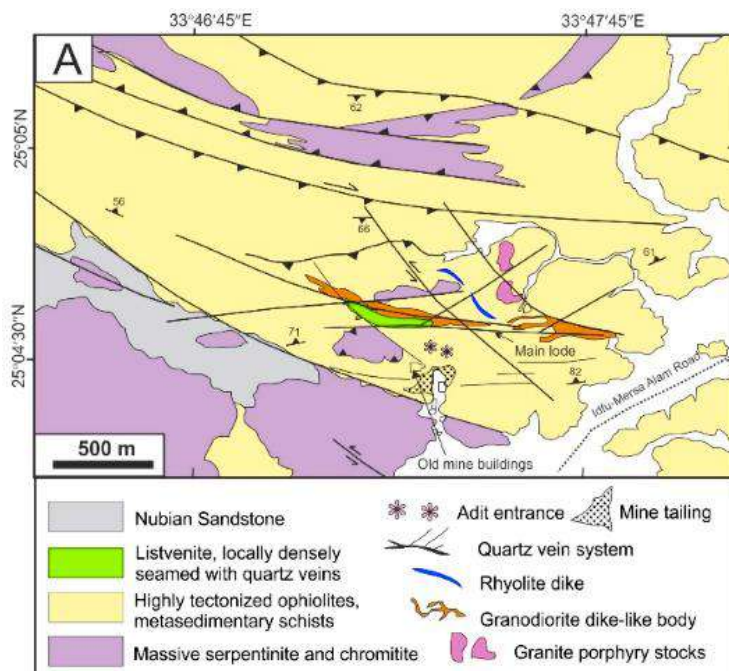
Figure 4. Detailed geological map of selected gold occurrences/deposits in the Barramiya (Egypt deposit area). The Barramiya gold deposit is expressed in auriferous quartz and quartz–carbonate veins. 36
